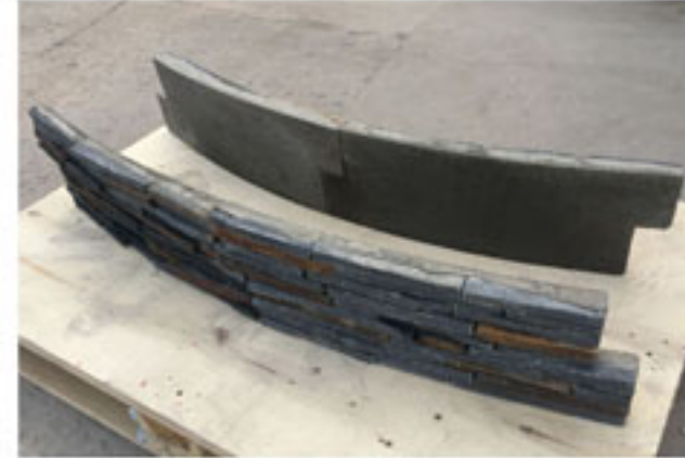
1) Both the Internal and External Curved Panels are available for your reference.
